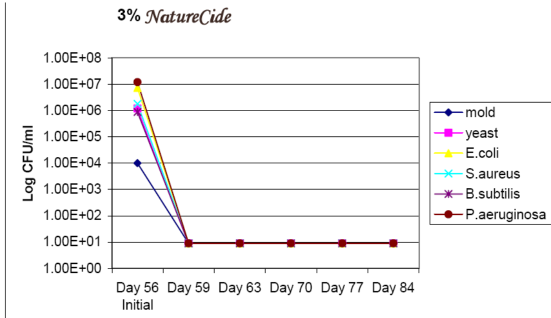
Figure 3. On Day 56, the same 3% NatureCide Extract solution was re-inoculated with the selected microorganisms.
