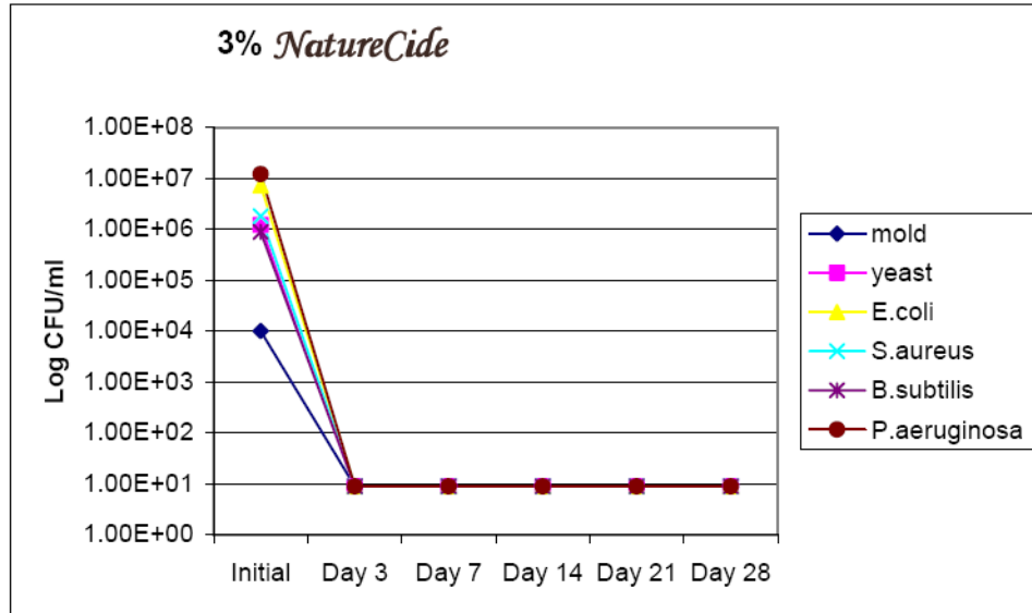
Figure 1. On Day 0, a 3% NatureCide Extract solution was inoculated with the selected microorganisms.
