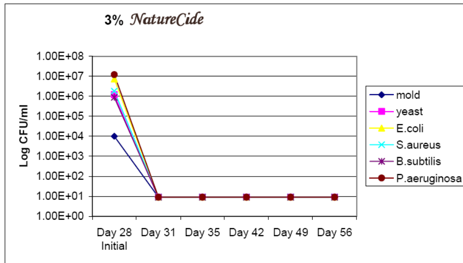
Figure 2. On Day 28, the same 3% NatureCide Extract solution was re-inoculated with the selected microorganisms.
